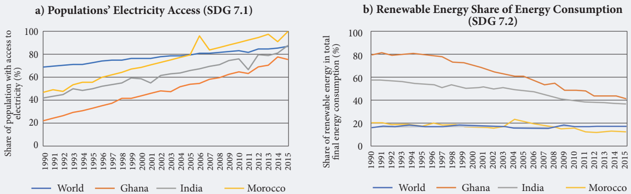
Figure 2. 1990-2015 Worldwide Trends and Those for Three Case Studies: Ghana, India and Morocco
